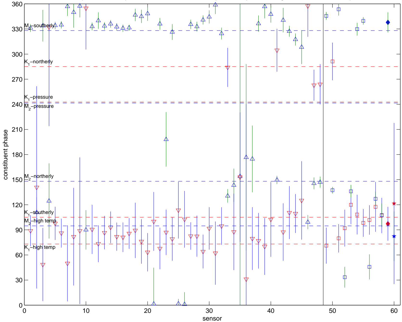
Greenwich Phases of Dominant Tidal Signals Tidal Constituents M2 in Blue, K1 in Red, Triangles denote Array Deployment 4 Jun–13 to May–14 Squares are Tempo t-chain, Diamond denotes Optode Temp and Pentagram denotes RAS Temp
